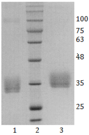
Figure 1. SDS-PAGE analysis of human DNase I visualized by PageBlue protein staining solution (Fermentas). Lane 1. 2 µg of hDNase I (non-reduced); Lane 2. Protein size marker ( Prestained protein ladder, 8003, Naxo); Lane 3. 2 µg of hDNase I (reduced).
