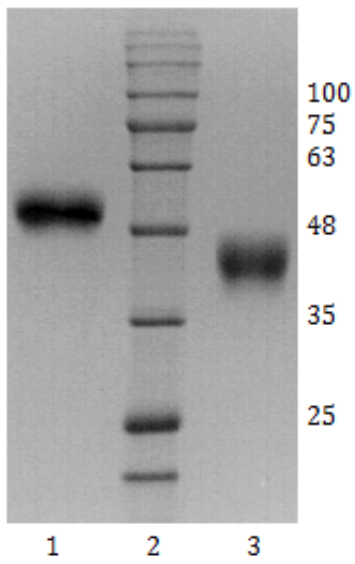
Figure 1. SDS-PAGE analysis of human GFRA-1 visualized by PageBlue protein staining solution (Fermentas). Lane 1. 2 µg of human GFRA-1 (reduced); Lane 2. Protein size marker ( Prestained protein ladder, 8003, Naxo); Lane 3. 2 µg of human GFRA-1 (non-reduced).
