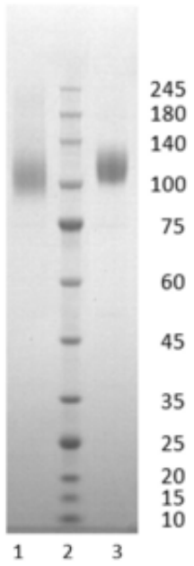
Figure 1. Coomassie-stained SDS-PAGE analysis of SARS-CoV-2 Spike S1 Indian B.1.617.2. 4-12% gradient gel is used for analysis. Lane 1. 0.8 \mu g SARS-CoV-2 Spike S1 Indian B.1.617.2 (-DTT) Lane 2. Protein marker (Smobio) Lane 3. 0.8 \mu g SARS-CoV-2 Spike S1 Indian B.1.617.2 (+DTT).
