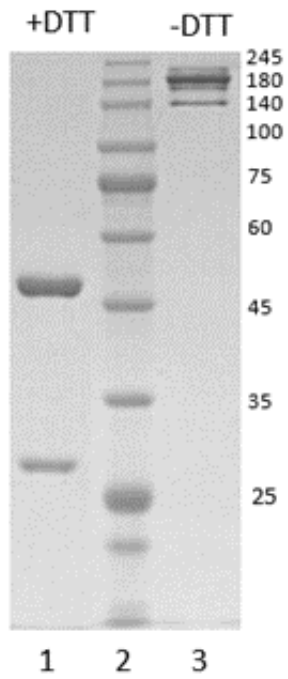
Figure 1. Coomassie-stained SDS-PAGE analysis of monoclonal antibody to SARS-CoV-2 Spike RBD, clone 60E10. 10% gel is used for analysis. Lane 1. Monoclonal antibody to SARS-CoV-2 Spike RBD, clone 60E10 (+DTT). Lane 2. Size marker. Lane 3. Monoclonal antibody to SARS-CoV-2 Spike RBD, clone 60E10 (-DTT).
