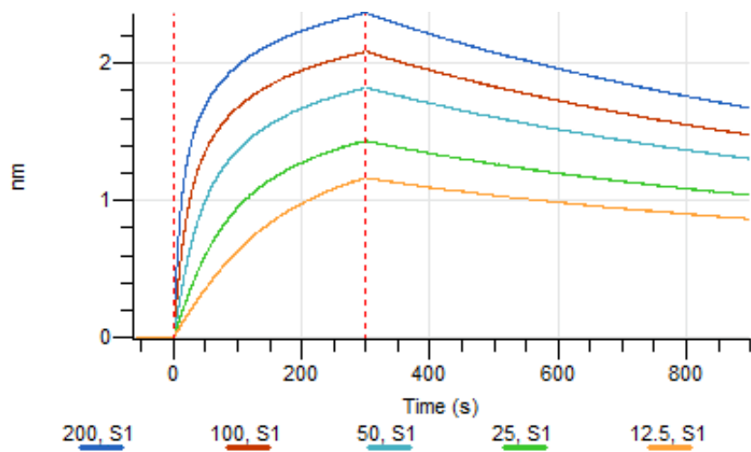
Figure 4. Octet RED96e analysis, antibody was loaded on sensor for capture of Spike S1 protein in different concentrations: 200 nM, 100 nM, 50 nM, 25 nM and 12.5 nM.
