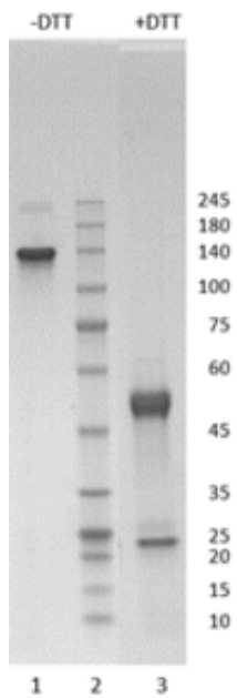
Figure 1. Simply Blue Safe stained SDS-PAGE analysis of monoclonal antibody to SARS-CoV-2 Nucleocapsid protein, clone 82C3. 4-12% gradient gel is used for analysis. Lane 1. Monoclonal antibody to SARS-CoV-2 Nucleocapsid protein, clone 82C3 (-DTT). Lane 2. Size marker. Lane 3. Monoclonal antibody to SARS-CoV-2 Nucleocapsid protein, clone 82C3 (+DTT).
