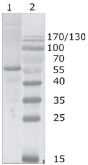
Figure 1: Western Blot testing of HIV-1 p24 antibody, clone N29. Line 1. HIV-1 Gag p17/24 (Han-2 subtype) Line 2. Protein size marker.
