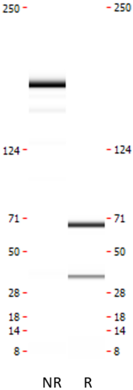
Figure 1. CE-SDS virtual gel output (LabChip GX) for monoclonal antibody to PAI-1, clone 3C3 under non-reduced (NR, left) and reduced (R, right) conditions.
